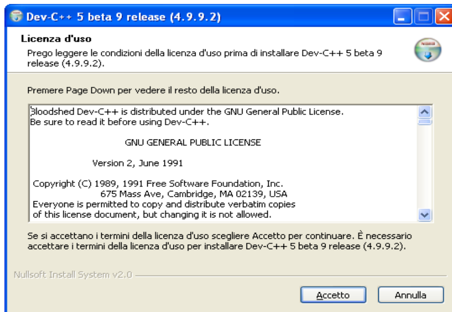
Fig. 2.1: License Agreement
